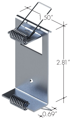
MB-WPS-S Metal spring clip mounting bracket
