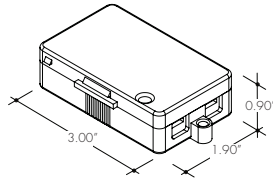
LVSP-4T-BK Low Voltage, 4 Terminal Splice Box, Black
