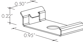
MB-KXLC-SS Stainless steel screw-in mounting bracket
