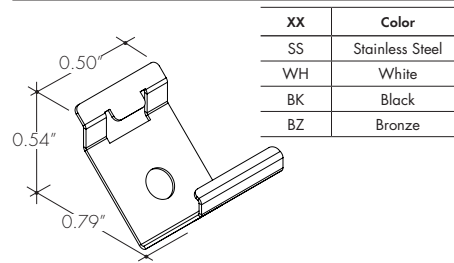
MB-KMSC-45-XX Fixed mounting clip 45° -FC45
