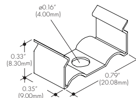
MC-07XXC Mounting clip
