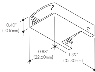
HG-0704C Flex connect auxiliary housing accessory
