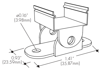
RC-07XXC Rotating mounting clip
