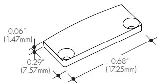
EC-0704C-H0 Silver Anodized End Cap
