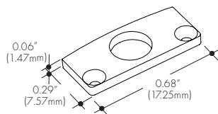
EC-0704C-H1 Silver Anodized End Cap with powerfeed opening
