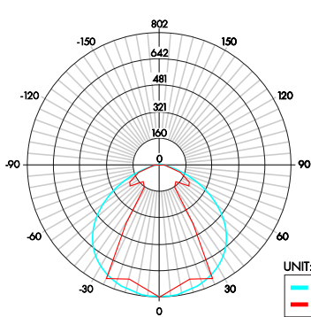
K45M-48-30K-VHO-C-XX
