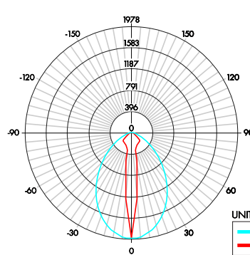
K45M-48-30K-VHO-13-XX
