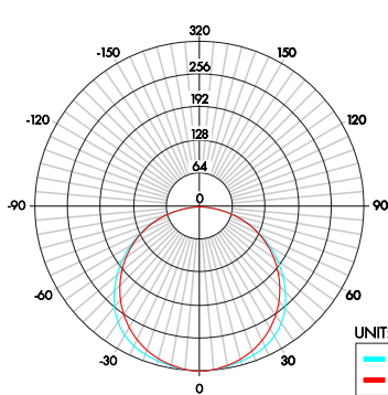
K45M-48-30K-VHO-F-XX
