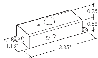
Male Quick Connect, FMA, LMC, LYC, or IS-DC are required for input and output.
