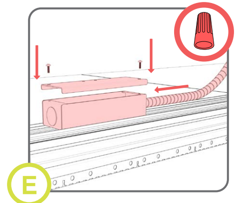
Secure BX cable to junction box and make electrical connections. Screw cover in place. Fixez le câble à la boîte de jonction. Fixez le couvert en place.
