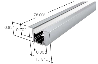
MC-FS-KBL-F-V-78 Flanged Mounting Channel with grip, 78"
