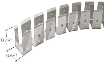
MC-BNS-KBL-F-V-34 Bendable Mounting Channel with grip, 34"
