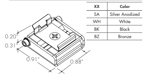
MB-KXLC-A.-XX Adjustable mounting clip -A
